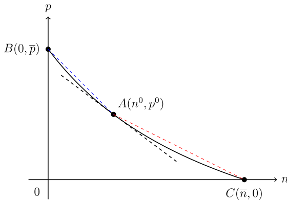
Fig. 1. Essence of the proof.
